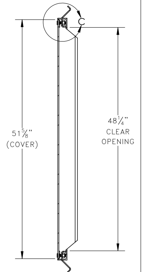
SECTION B-B
