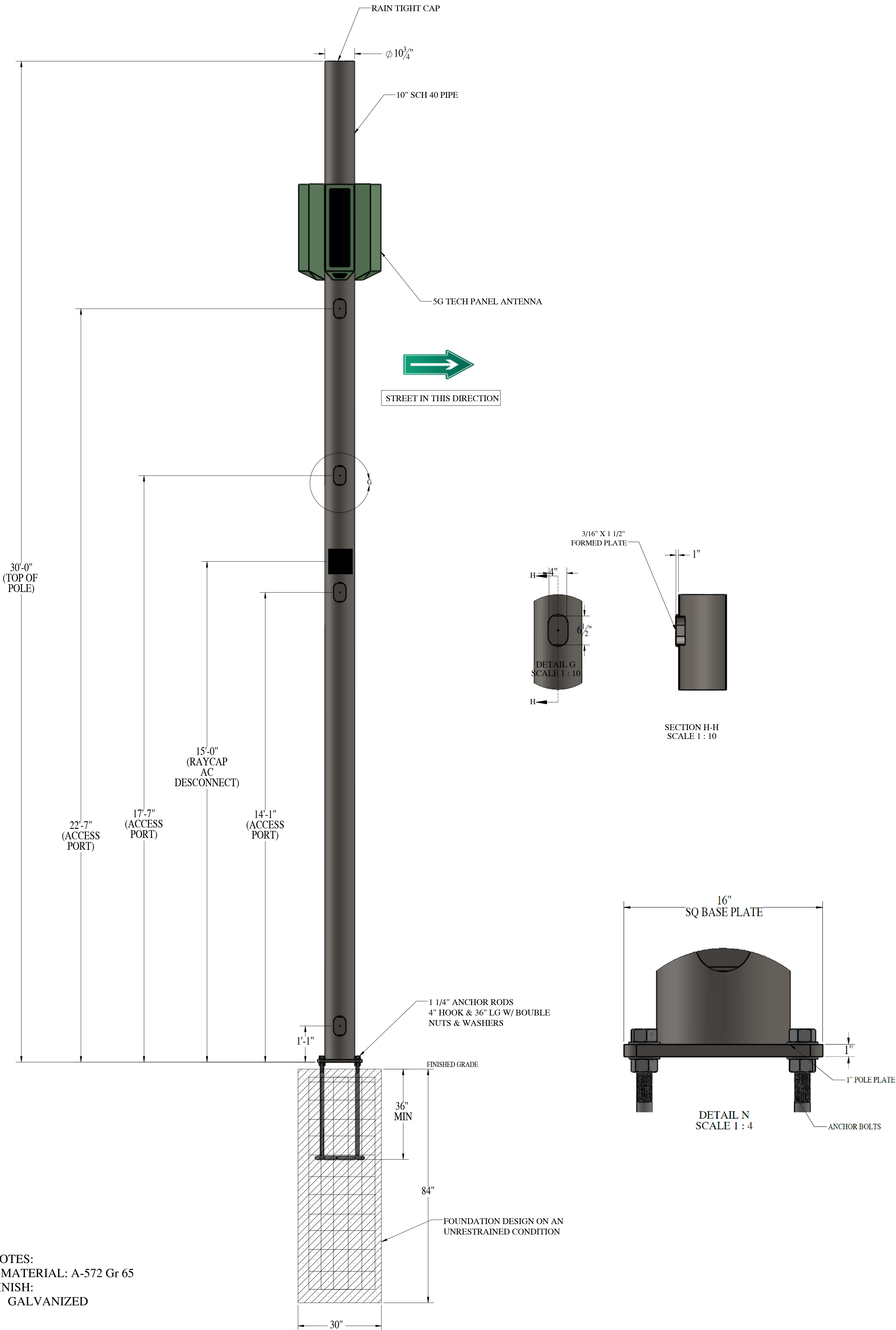
ELAVATION VIEW
