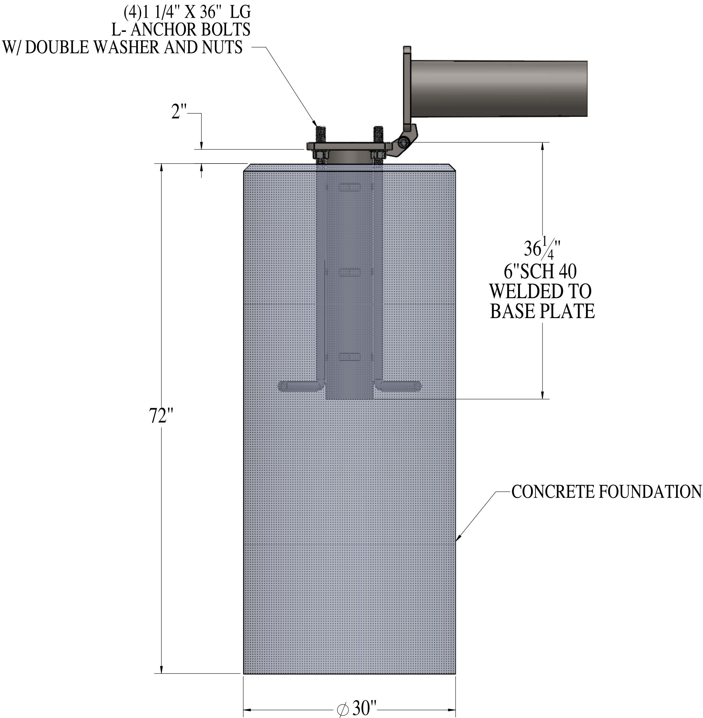
FOUNDATION VIEW
